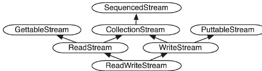
Fig. 2. The ANSI Smalltalk standard stream protocol hierarchy.
