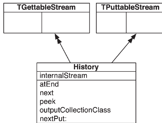
Fig. 7. The class History.
