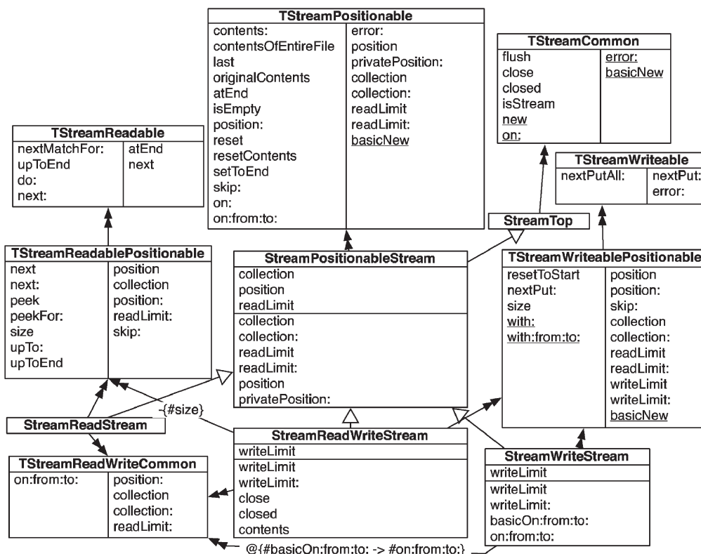
Fig. 13. Schärli's refactored stream hierarchy.
