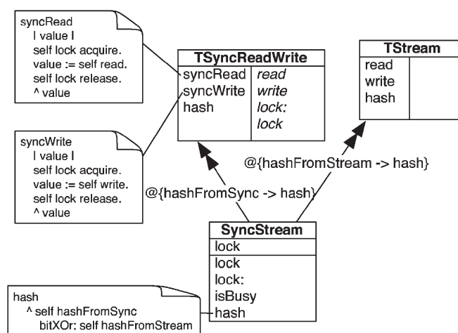
Fig. A1. The class SyncStream is composed of the two traits TSyncReadWrite and TStream.
