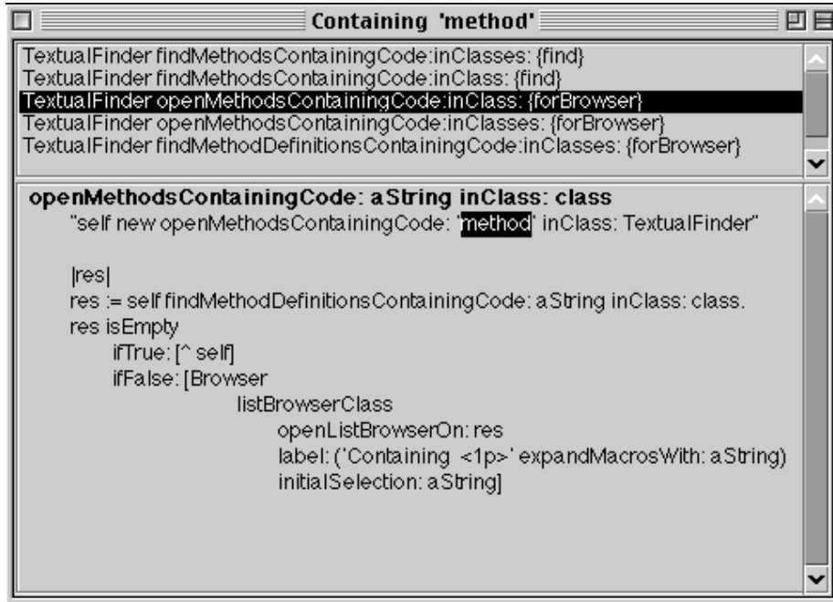
Figure 1: The result of the textual finder on a query looking for 'method' in the TextualFinder itself.
