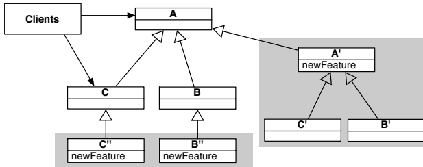
Figure 2: Two strategies (gray portions) to introduce changes without impacting existing clients
