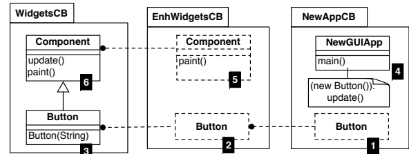
Lookup of update when new Button().update() is performed in NewAppCB: 1, 2, 3, 4, 5, 6. The method update calls the method paint. The latter is looked up as: 1, 2, 3, 4, 5.
