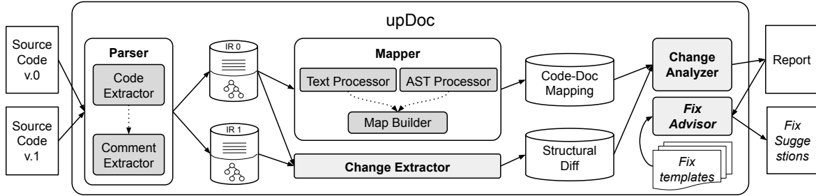
Fig. 1. upDoc workflow diagram
