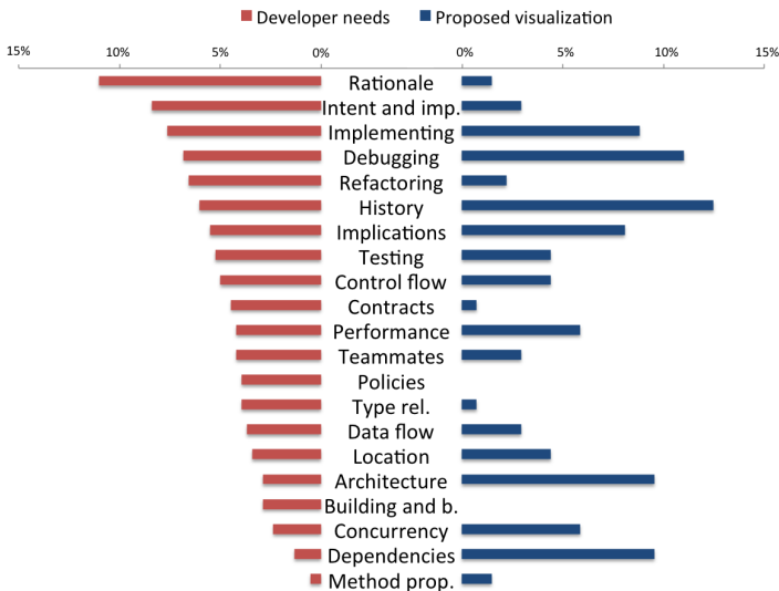
Figure 2.10: Problem-oriented analysis of importance of developer needs vs. their visualization support. Ideally, both charts would be symmetrical. However, we observe several unbalanced domains.
