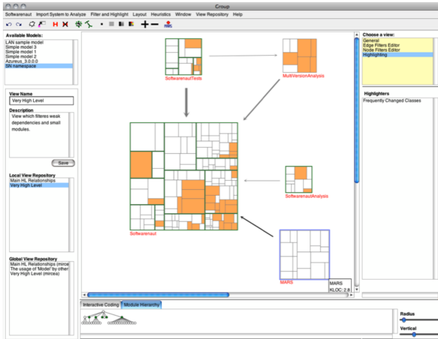
Figure 4.9: The SoftwareNaut tool for visualization of hierarchical structures to support architecture tasks.
