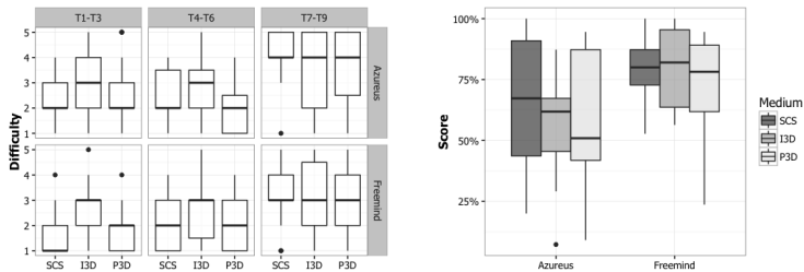
(a) Difficulty experienced by participants. Box plots are vertically grouped by the theme of tasks. The overall difficulty is higher in Azureus than in Freemind.
