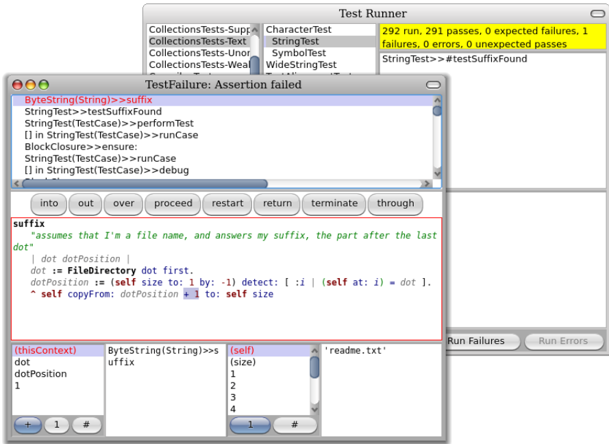
Figure 6.31: Changing the suffix method in the debugger: fixing the off-by-one error after an SUnit assertion failure
