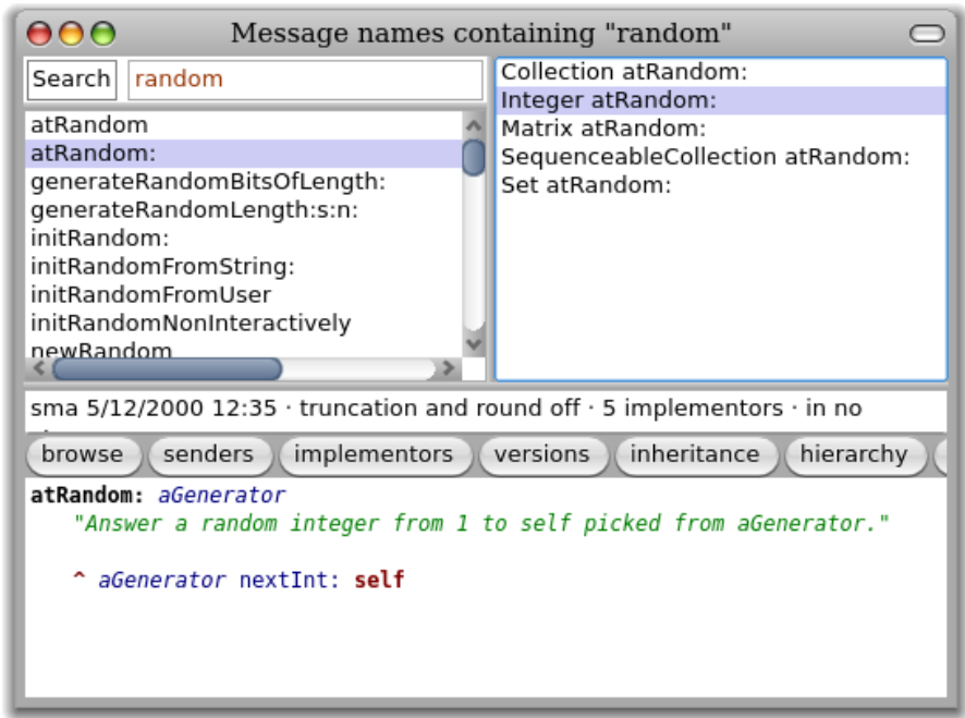
Figure 6.33: The message names browser showing all methods containing the substring random in their selectors.
