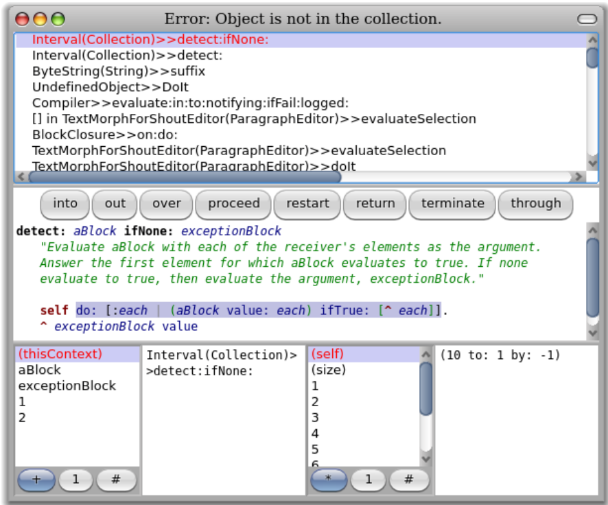
Figure 6.28: The debugger after restarting the detect:ifNone: method
