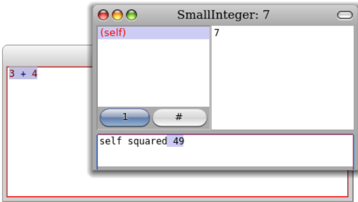
Figure 1.10: Inspecting an object.
