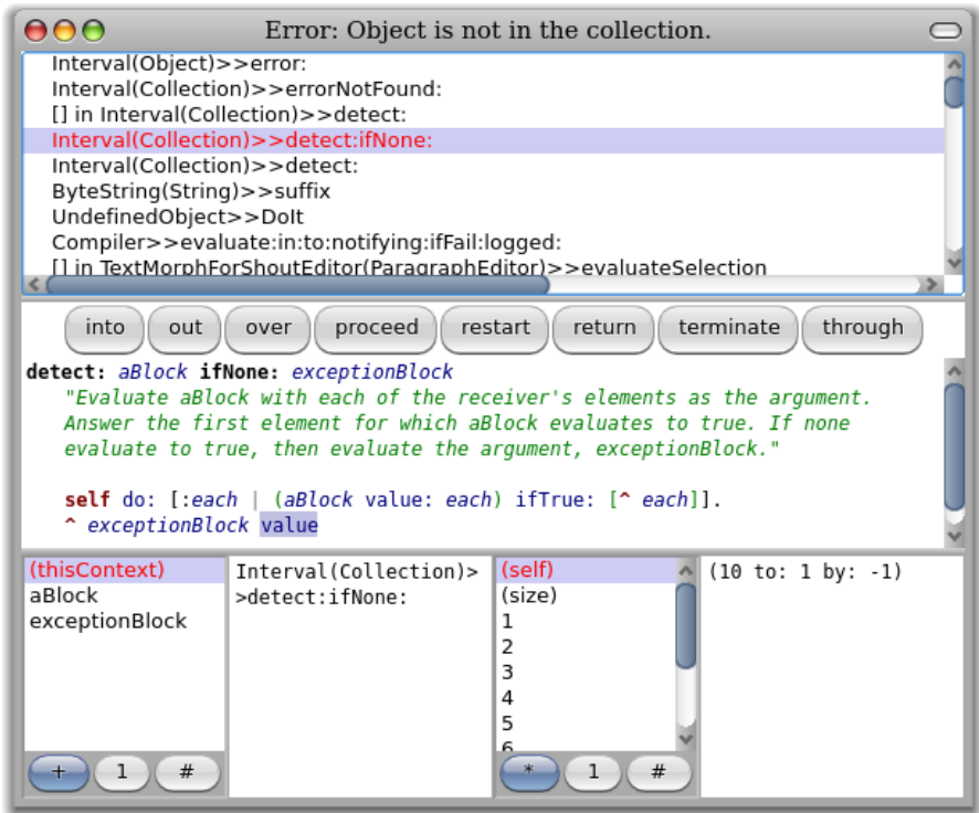
Figure 6.27: The debugger.
