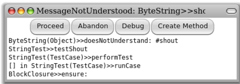
Figure 1.22: The (pre-)debugger.
