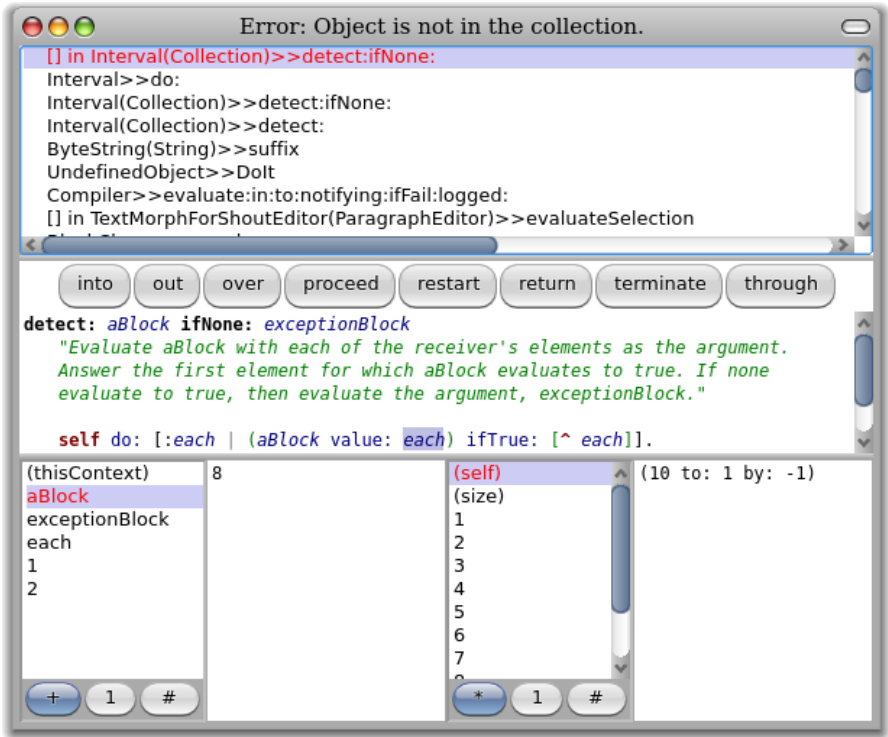
Figure 6.29: The debugger after stepping Through the do: method several times.
