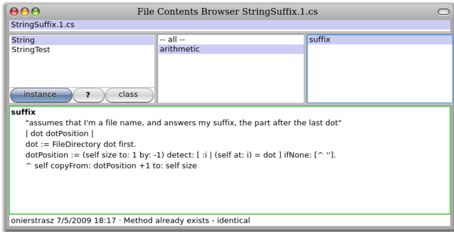
Figure 6.36: A File Contents Browser
