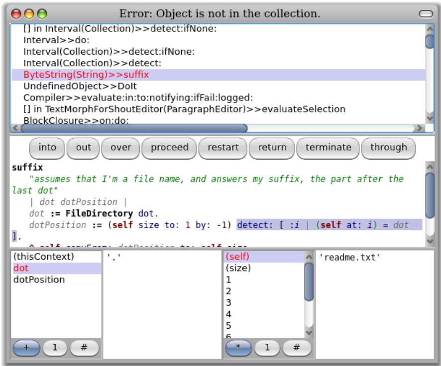
Figure 6.30: The debugger showing why 'readme.txt' at 7 is not equal to dot
