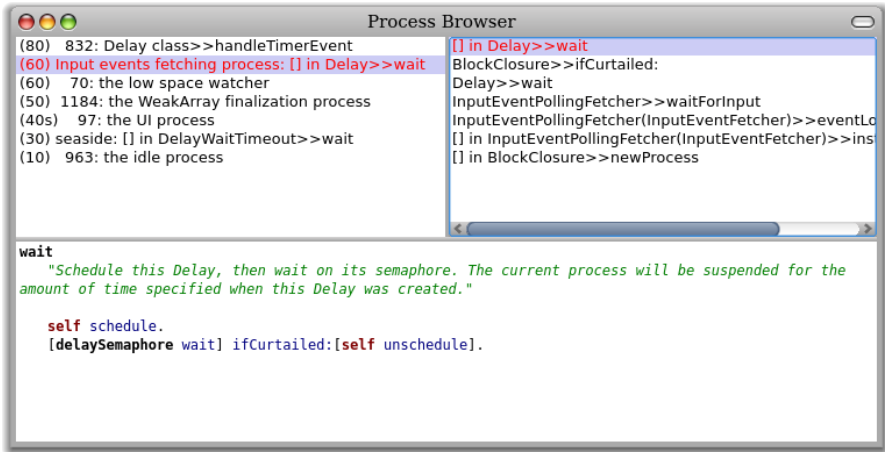
Figure 6.32: The Process Browser
