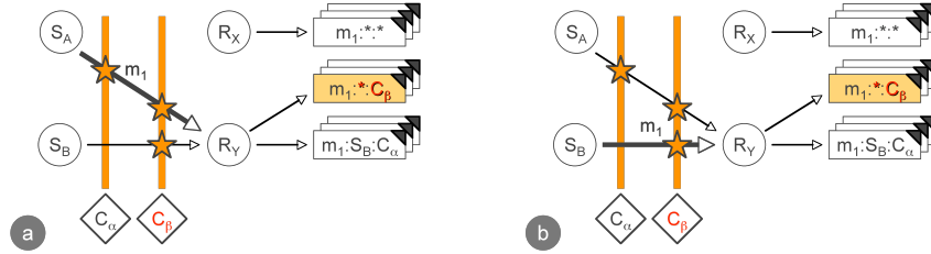
Figure 3: Four-dimensional method dispatch.
