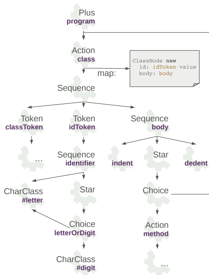
Figure 6.1: The structure of parser combinators created after evaluating the code of Listing 6.1.
