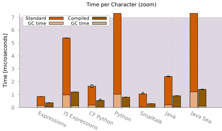
Figure F.4: Time per character of plain PetitParser and its compiled version for different grammars, the zoomed-in version.
