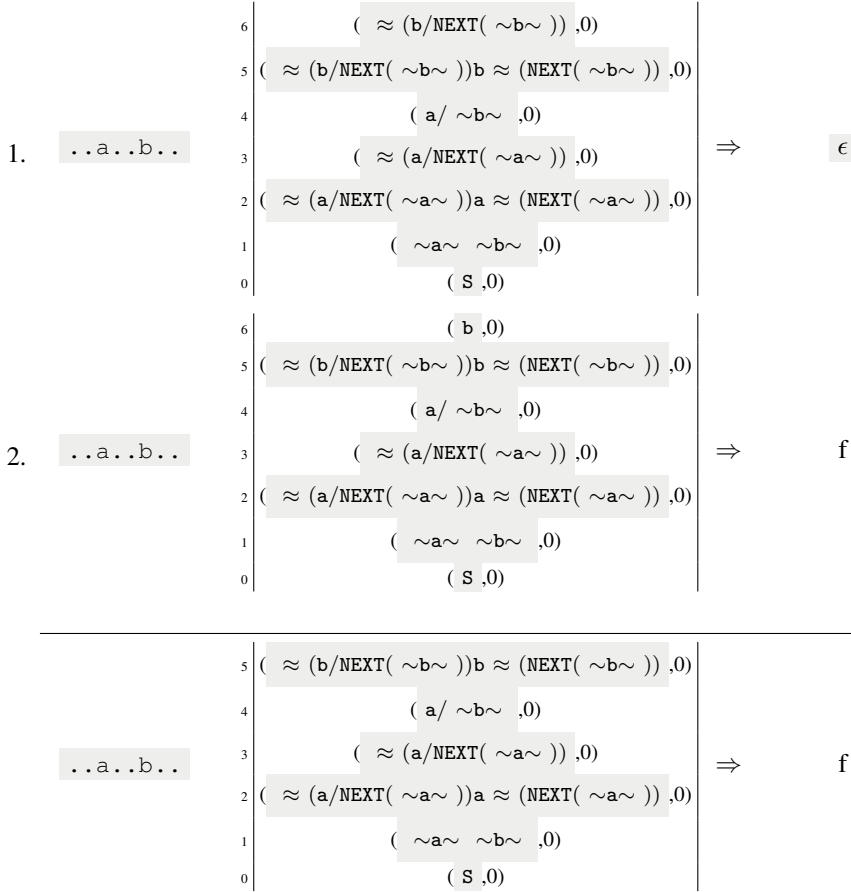
Figure B.15: The inference rule for sequence (failure case).
