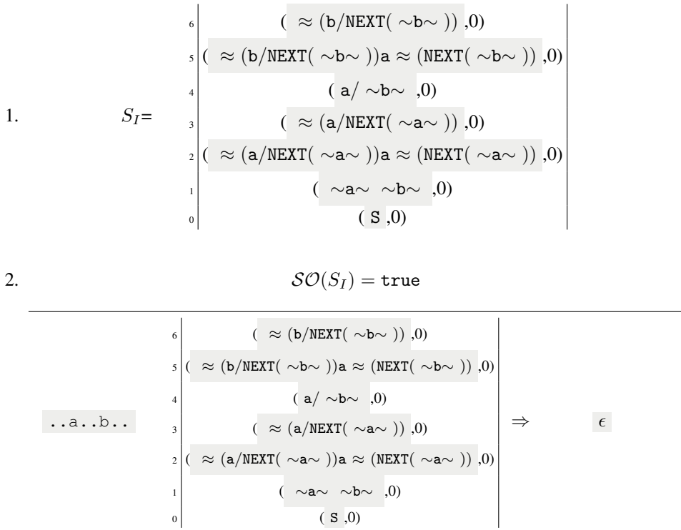
Figure B.16: The inference rule for overlapping seas.
