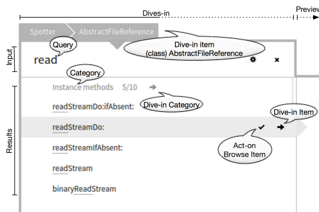
Fig. 1. SPOTTER UI is composed of an input field for queries, results, preview, and dives-in bar that indicates where a user searches for. The results are structured into categories. The user can dive-in a category or a selected item, or can act-on the selected item (by pressing the enter key) that usually opens the selected item in a specific tool.
