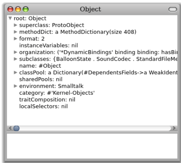
Figure 1.11: Exploring Object.
