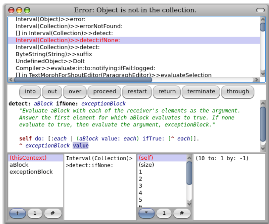
Figure 6.27: The debugger.
