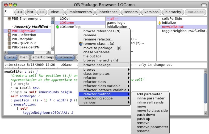
Figure 6.13: Refactoring operations.
