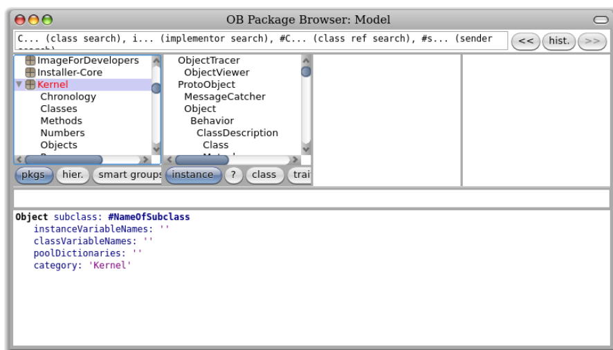
Figure 6.5: Browser showing the method-creation template
