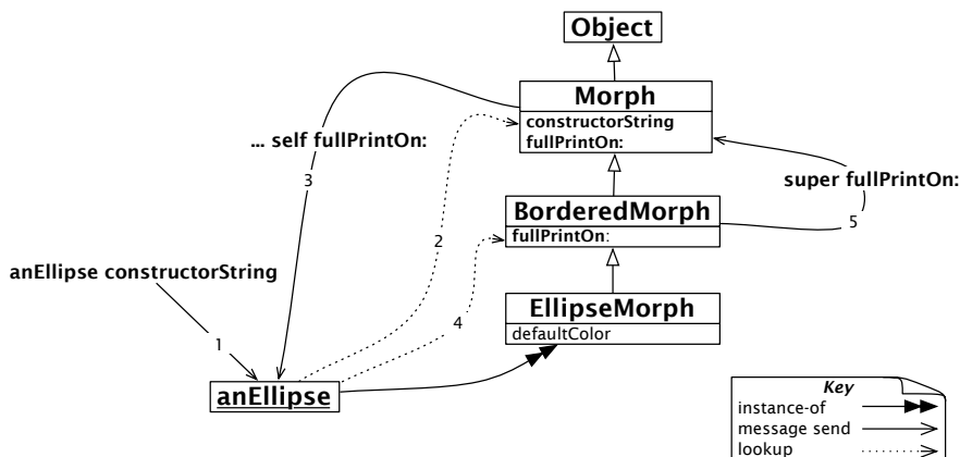
Figure 5.3: self and super sends
