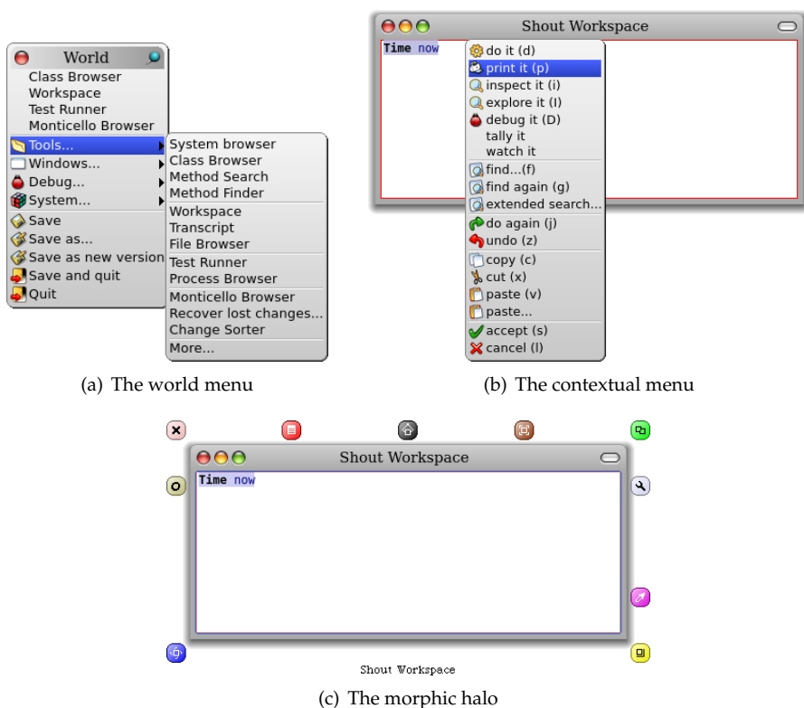
Figure 1.3: The world menu (brought up clicking), a contextual menu (action-clicking), and a morphic halo (meta-clicking).
