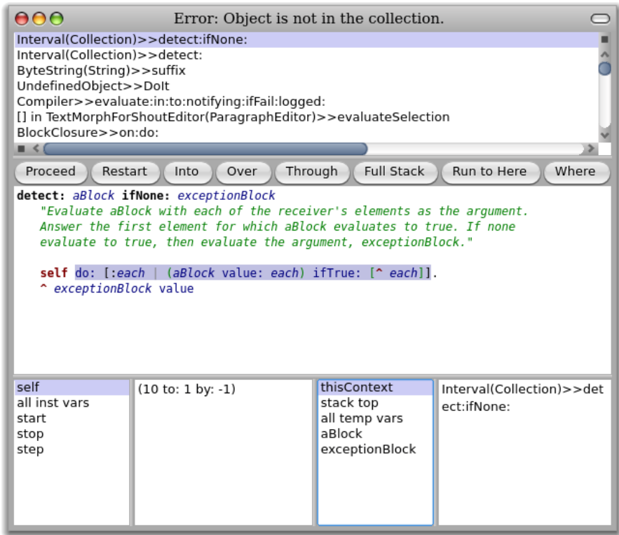
Figure 6.28: The debugger after restarting the detect: ifNone: method
