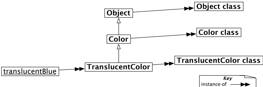
Figure 13.3: The metaclasses of Translucent and its superclasses
