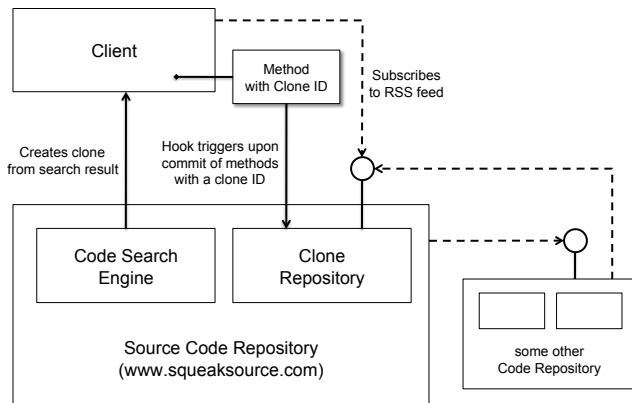
Figure 1: Proposed architecture of the “hot clone” prototype. It extends Monticello, a distributed version control system for Smalltalk, with two components: a code search engine and a clone repository.
